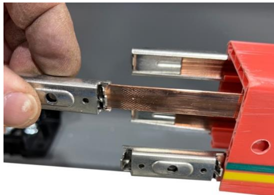
4.6.3 Adding the Copper Splice Connector
