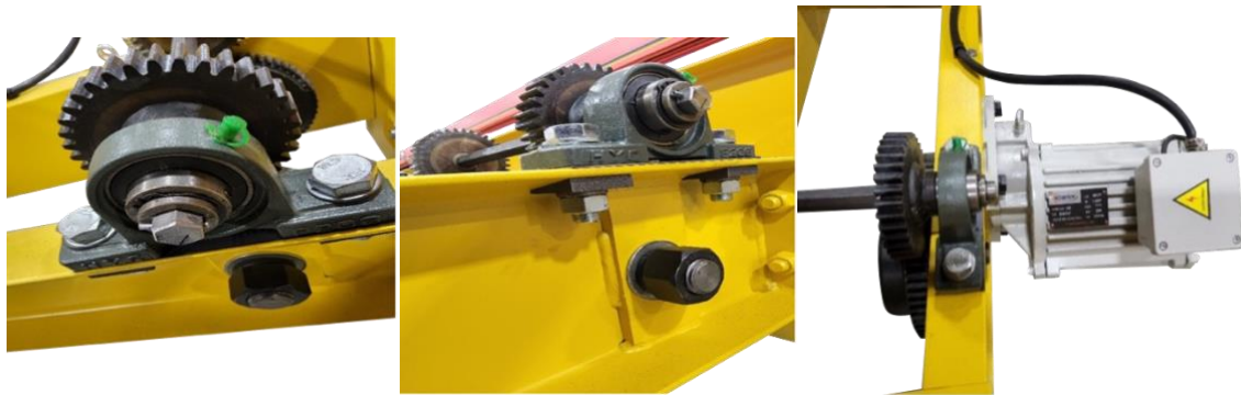
4.6.4 Gears
