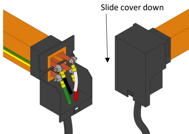
Image 7.13 Attached Wires
