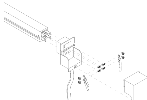
Image 7.14B Supply Box Exploded View
