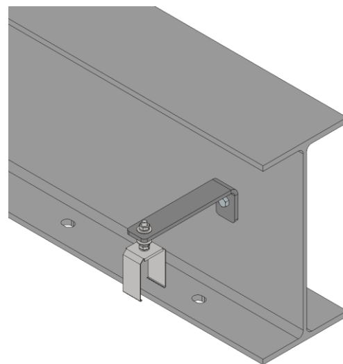
Image 7.1C Bolted Brackets
