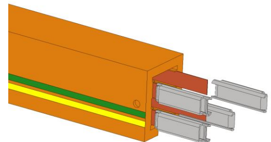
Image 7.6 Conductor Couplers
