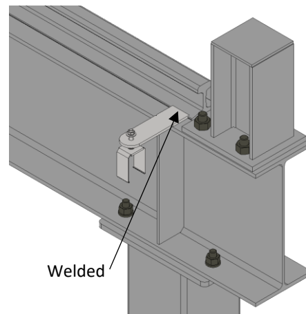
Image 7.1A Welded Brackets
