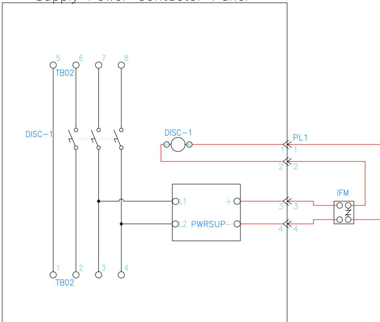
Supply Power Contactor Panel
