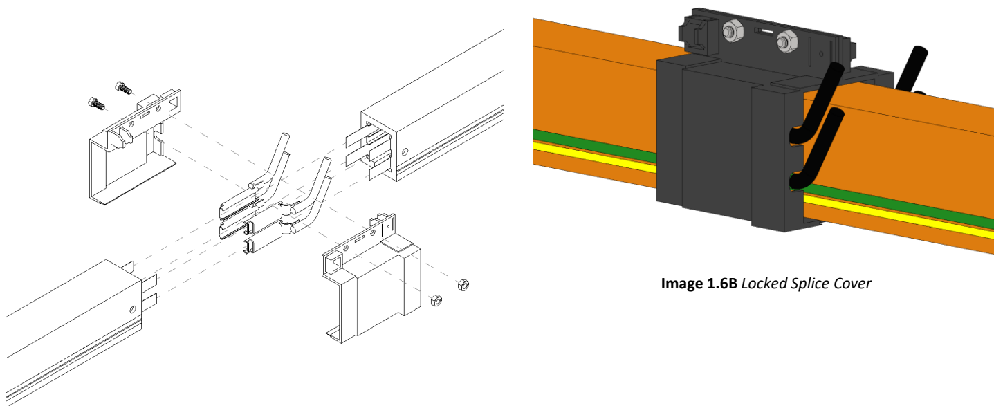
Image 1.6A Splice Cover Exploded View
