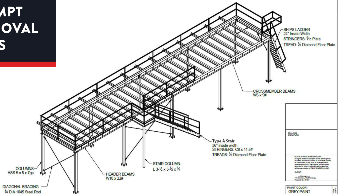
Closed Tread - 3 Rail + Inner Hand Rail
